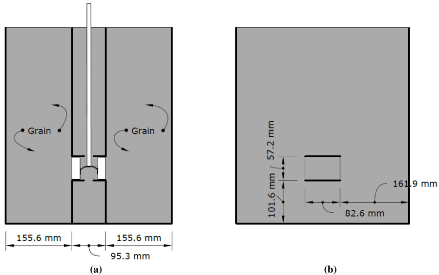
Figure 2. (a) Cross-section of the welded box showing how the blocks are connected to the rod and how they push the grain and (b) one of the interior panels showing the location of the rectangular hole.
