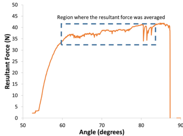
Figure 5. Sample force curve showing the region used to calculate the average force. The angle ( \theta ) on the x -axis is defined in figure 4.
