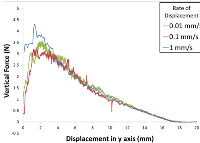
Figure 3. Comparison of different displacement rates for measurement of the friction coefficient of steel.
