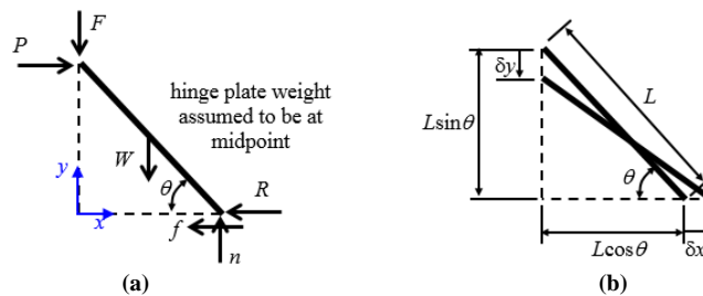
Figure 4. Free-body diagrams of one of the two hinge side plates showing the forces applied by the rod and wooden block.
