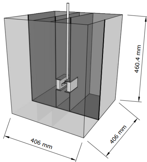
Figure 1. Welded box designed to measure passive grain pressure. The rod is attached to a load cell on a Criterion testing machine (not shown). As the Criterion machine pushes the rod downward, the hinges push the blocks horizontally.
